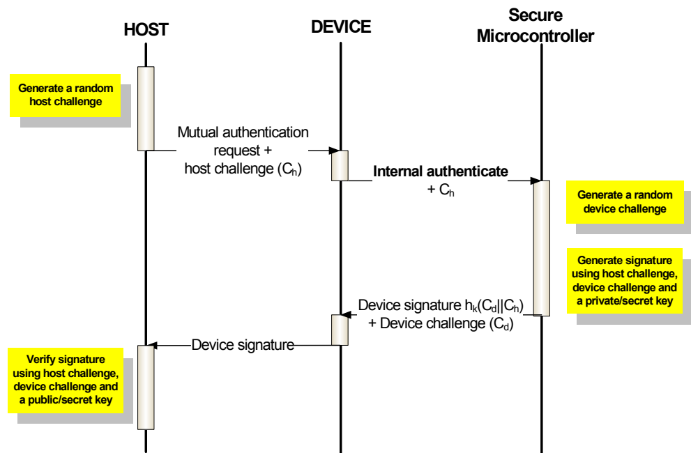
Figure 4-1. Challenge-response unilateral authentication
