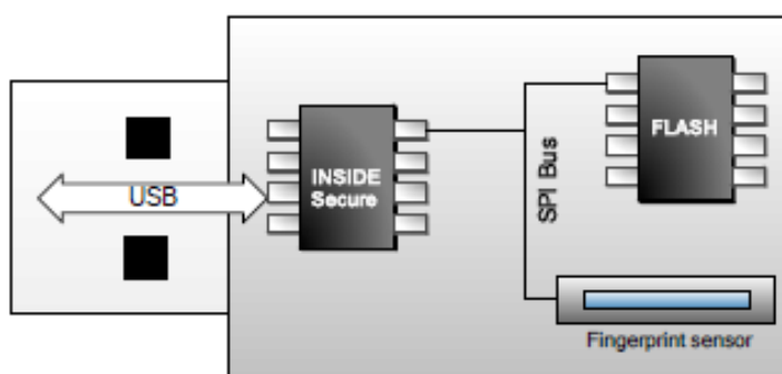
Figure 4-3. OTP-enabled, mass storage biometric USB token
