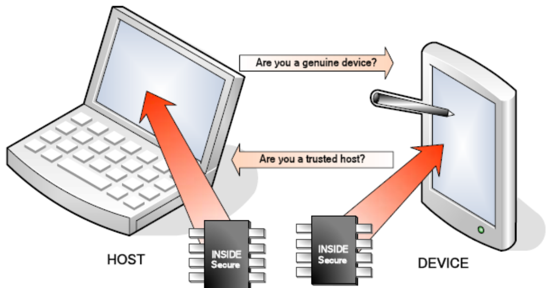
Figure 2-1. Authentication
